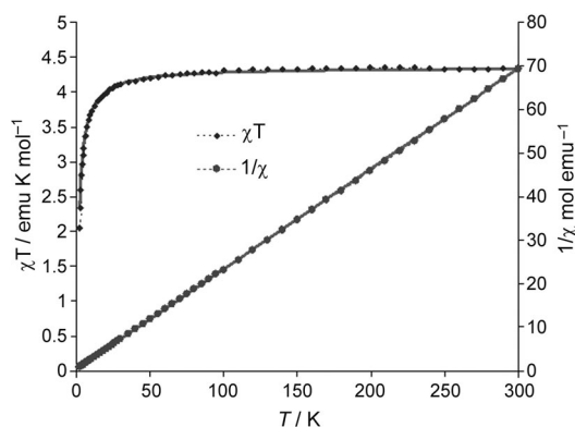
Figure 4. Temperature dependence of \chi T for 1 (diamonds) and 1/\chi (circles). The solid lines are the best fit to the Curie–Weiss law.
